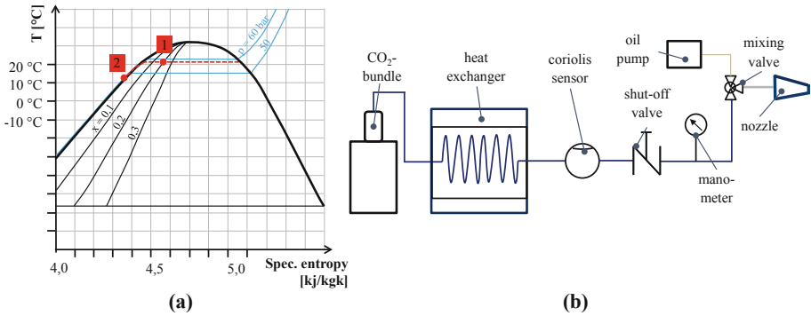
Fig. 3. a. T-s diagram \text{CO}_2 . b. experimental setup.
