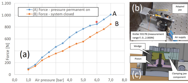
Fig. 8. (a) Forces as a function of air pressure level (*identical to manufacturer's specification). (b) Force measurement set-up for a single jaw. (c) The pneumatic chuck with central piston and wedge acting on the three jaws.
