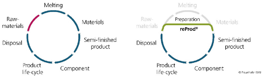
Fig. 3. The standard metal cycle and the smart shortened reProd ® cycle by cutting off the most energy-consuming and CO 2 -emitting process steps, such as melting and hot rolling.
