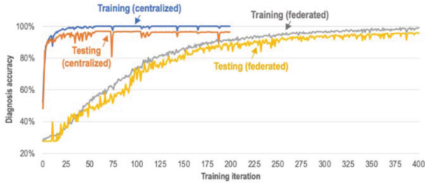
Fig. 4. Training and testing curves: centralized vs. federated scenarios
