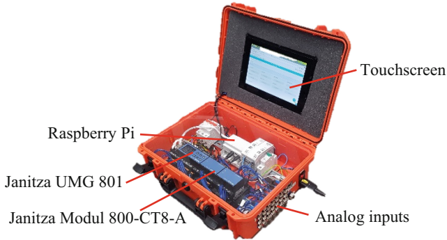
Fig. 2. Energy transparency and analysis system (ETAS).
