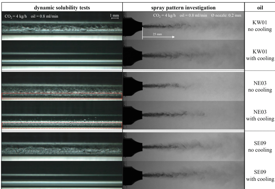
Fig. 5. Results of dynamic solubility and spray pattern tests
