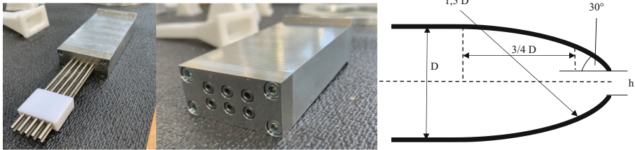
Fig. 1. Reference nozzles used; left: Needle nozzle; middle: Modular nozzle; right: Rouse-nozzle profile based on Rouse et al. and Webster et al. [12, 13]
