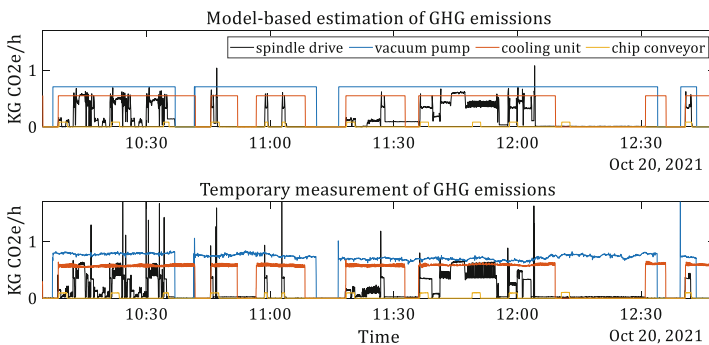
Fig. 4. Comparison between estimated and measured GHG emissions of selected auxiliary drives and the spindle drive
