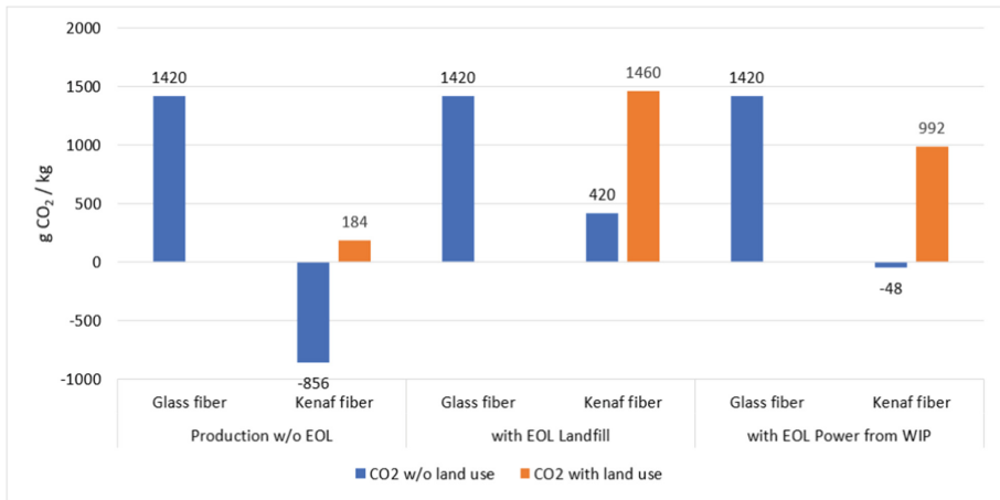
Fig. 3. Comparison of CO 2 emissions of glass fiber and kenaf fiber without and with accounting for land use as a missing CO 2 reservoir for 1 year.
