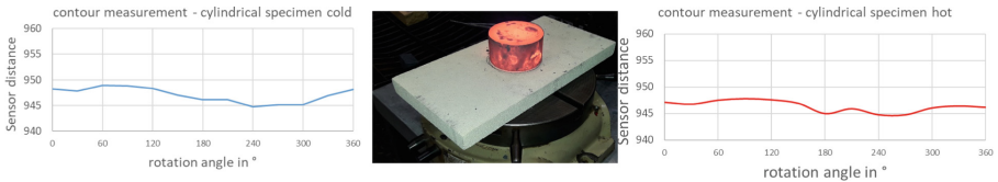
Fig. 8. Scenario >>Line<< - measurement cylindrical specimen
