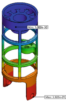
Fig. 2. Total deformation of link 1
