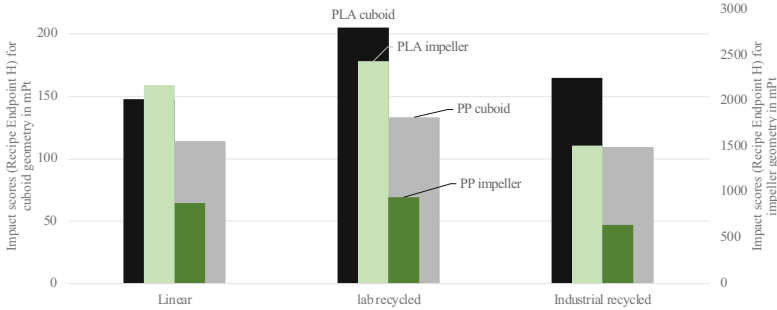
Fig. 6. Comparison of LCIA impact scores for PLA (left columns) and PP (right columns)
