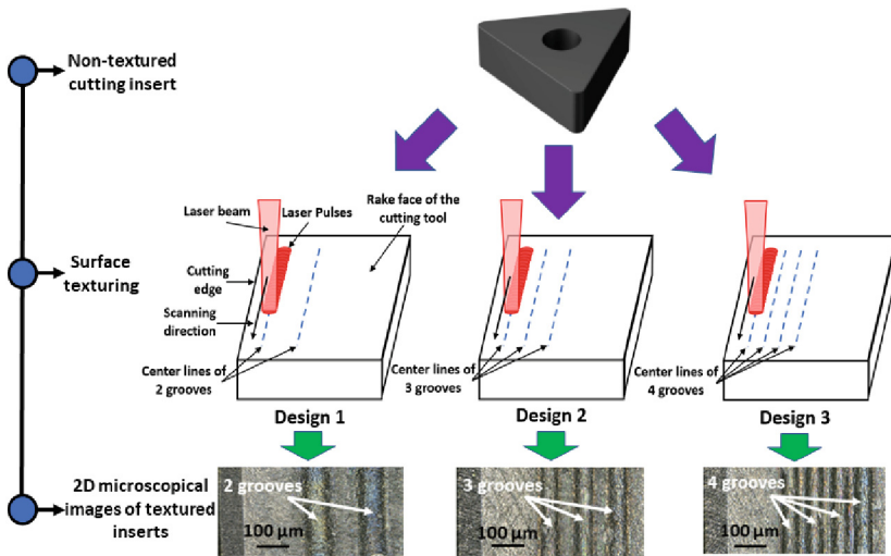
Fig. 1. A schematic showing the preparation process of the three different cutting tool designs
