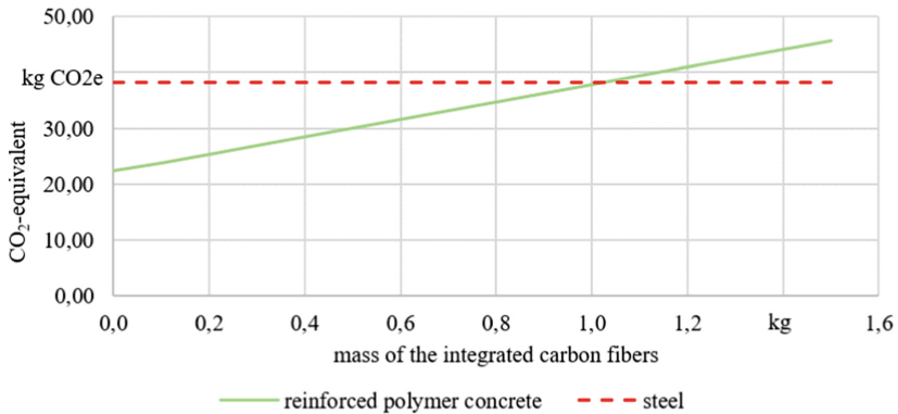
Fig. 7. CO 2 -equivalent of the extension arm made of fiber reinforced polymer concrete depending on the mass of carbon fibers compared to the CO 2 -equivalent of the steel extension arm
