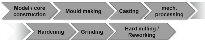
Fig. 3. Process chain for manufacturing the tool with cast cooling channels/sand core casting, based on [4]
