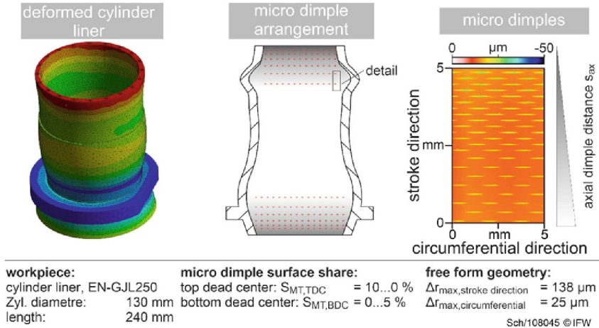
Fig. 2. Non-circularly machined cylinder liner with applied micro dimples (left graphic from Alshwawra, following [10])
