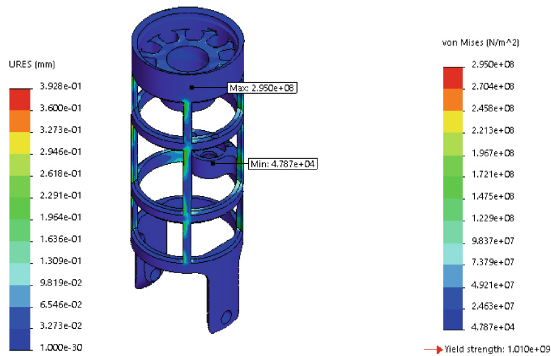
Fig. 3. Stress distribution of link 1
