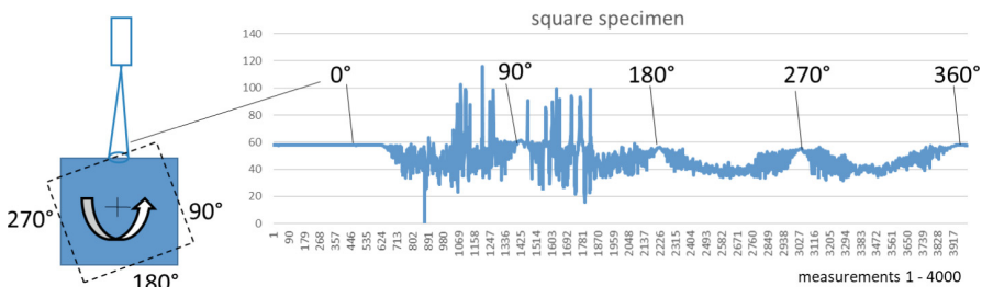
Fig. 6. Scenario >>Line<< - measurement square specimen
