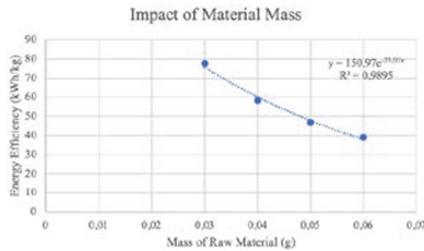
Fig. 5. Impact of raw material mass on the energy efficiency.
