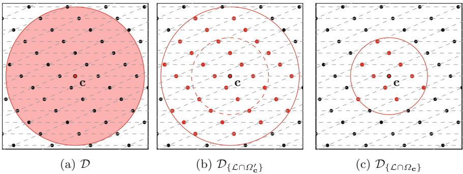
Fig. 2. Visual illustration of Algorithm 3. A continuous distribution is sampled (a), then discretized (b), and finally rejection sampling is applied (c).
