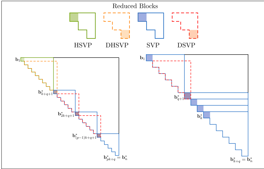
Fig. 2. Slide reduction of an upper-triangular matrix for n = pk + q \geq 2k (left) and n = k + q \leq 2k (right). (The original notion of slide reduction in [GN08a] used only SVP-reduced and DSVP-reduced blocks of fixed size k .)
