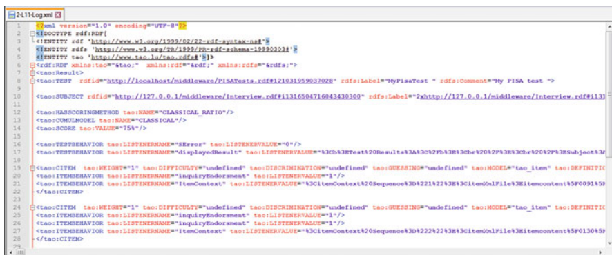
Fig. 10.2 Example of the appearance of a raw XML file
