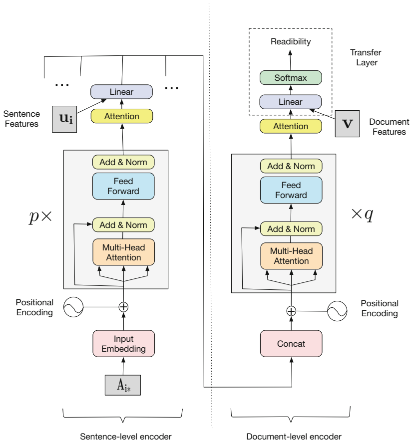
Fig. 1. ReadNet: proposed hierarchical transformer model specialized for readability analysis
