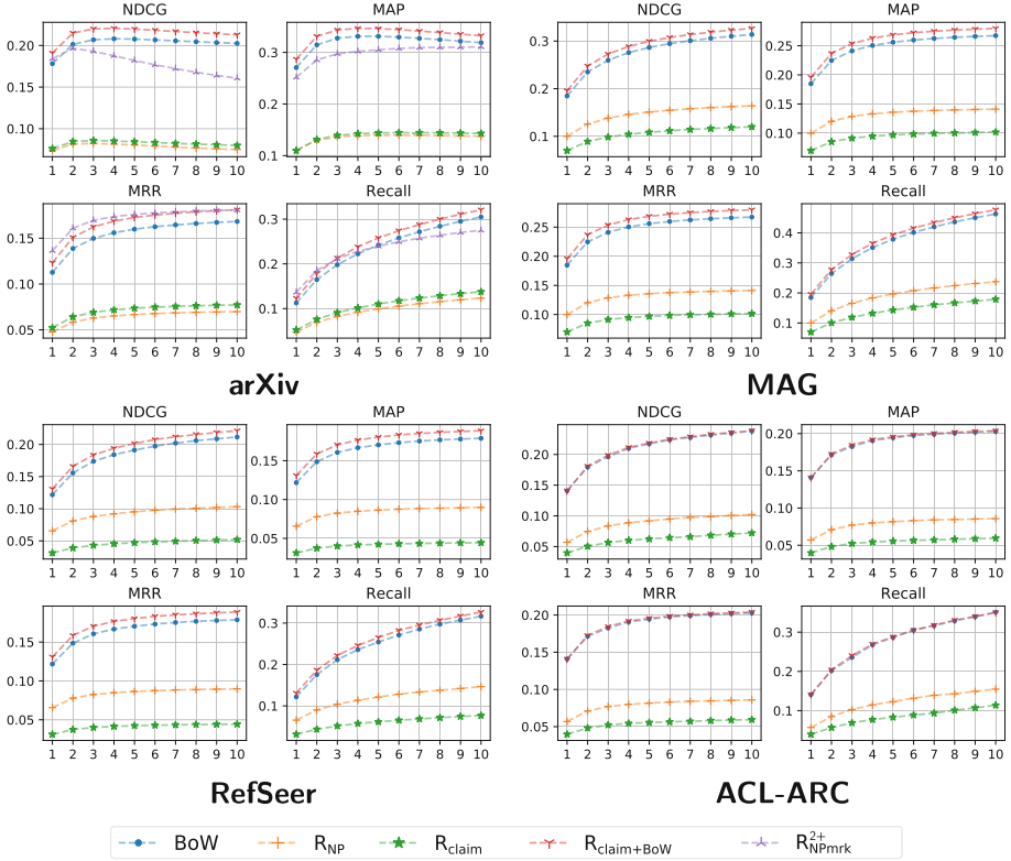
Fig. 2. Evaluation using arXiv, MAG, RefSeer and ACL-ARC. Showing NDCG, MAP, MRR and Recall scores at cut of values from 1 to 10.
