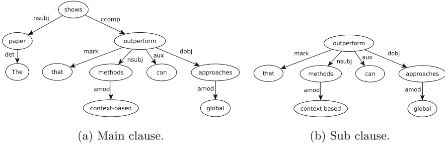
Fig. 1. UD trees as generated by PredPatt.
