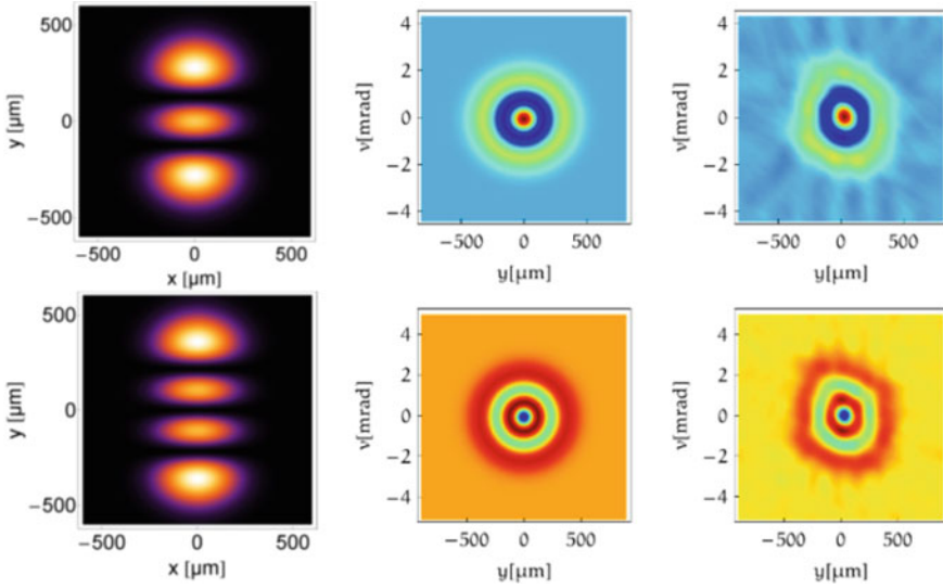
Fig. 20.10 Qualification of 4D Wigner formalism using near IR mode generator for different Hermite-Gaussian beams: Wigner distributions of TEM 02 and TEM 03 modes resulting from theory and experiment are shown for comparison
