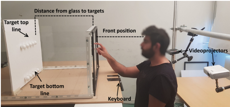
Fig. 5. Experimental setup.
