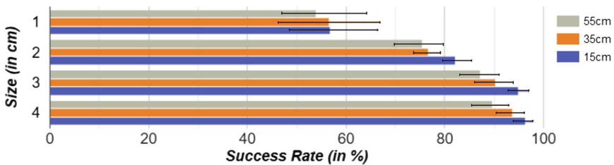
Fig. 7. Average success rate in % (with 95% CIs) according to target size and distance to the glass.
