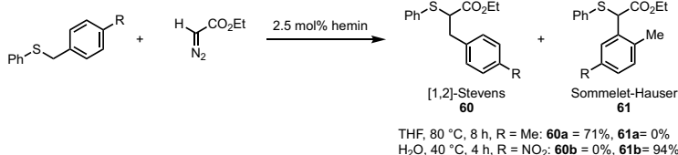
Scheme 50 Chemoselectivity between 1,2-migration and Sommelet–Hauser rearrangement
