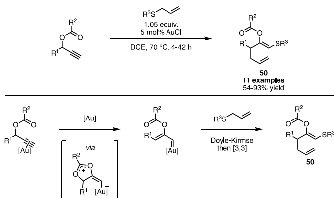
Scheme 43 Alkynes as masked ylides in Doyle–Kirmse chemistry
