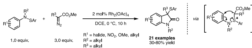
Scheme 35 Wang's modified Gassman oxindole synthesis
