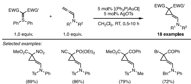
Scheme 14 Intermolecular cyclopropanation of allenamides
