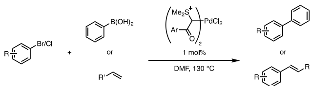
Scheme 1 Sulfonium ylides complexes as cross-coupling catalysts. DMF Dimethylformamide
