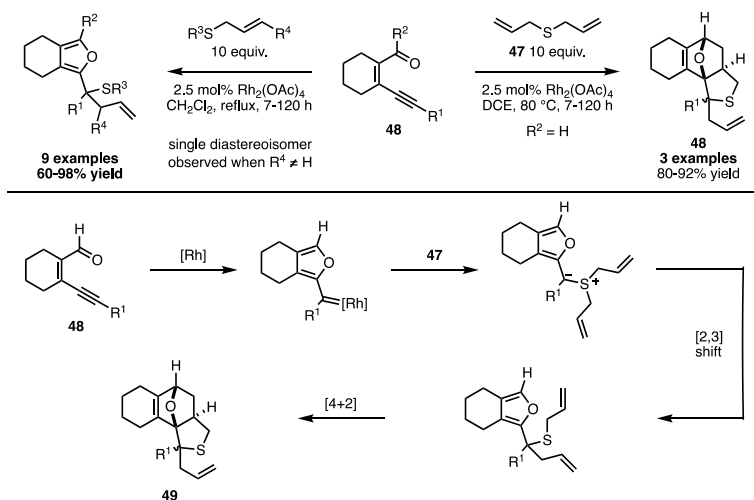
Scheme 42 Doyle–Kirmse reactions from in situ-generated (2-furyl)carbenoids
