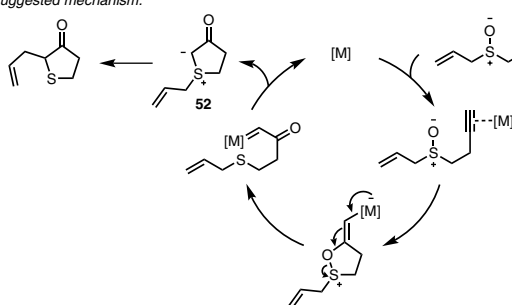
Scheme 44 Synthesis of sulfur heterocycles from alkynyl sulfoxides
