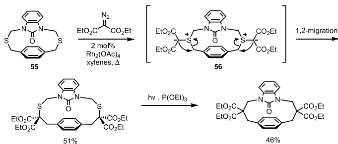
Scheme 46 Macrocyclic ring expansion by the double Stevens rearrangement
