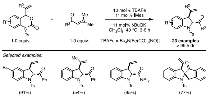
Scheme 5 Iron-catalysed decarboxylative formal (4 + 1) cycloadditions. TBAFe Bu 4 N[Fe(CO) 3 (NO)]
