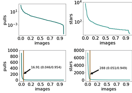
Fig. 4. Semilog pulls and stars distributions ( top ). Knee method ( bottom ).
