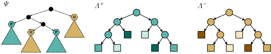
Fig. 1. Decision tree discriminating between popular and uncommon imagers (left), regression trees evaluating the popularity (center), and the degree of uncommonness (right). The regression trees are linked to corresponding leaves of \Psi : Regression trees like \Lambda^+ are linked to leaves marked with P ( popular ), while those like \Lambda^- to leaves marked with U ( uncommon ). (Best view in color)
