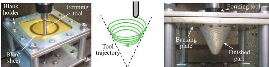
Fig. 1. Basic components to produce a cone by SPIF: (a) recently started process; (b) schema of the tool trajectory; and (c) finished sheet part.
