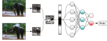
Fig. 4. The PickNet uses the flattened difference gray-scale image as input and produces a Bernoulli distribution to indicate picking the current frame or not.
