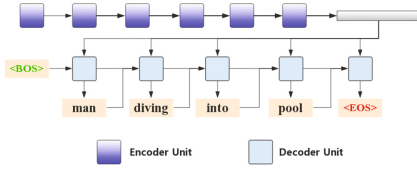
Fig. 3. The encode-decode procedure for video captioning.
