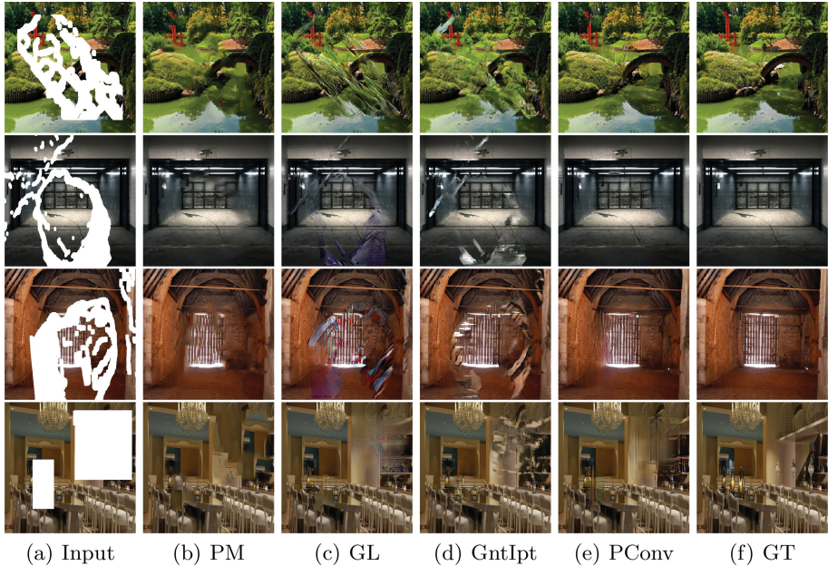
Fig. 6. Comparison of test results on Places2 images. (a) Input. (b) PM. (c) GL. (d) GntIpt. (e) PConv. (f) GT.
