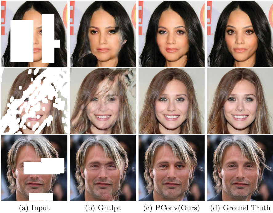
Fig. 9. Test results on CelebA-HQ. (a) Input. (b) GntIpt. (c) PConv (Ours). (d) Ground Truth.
