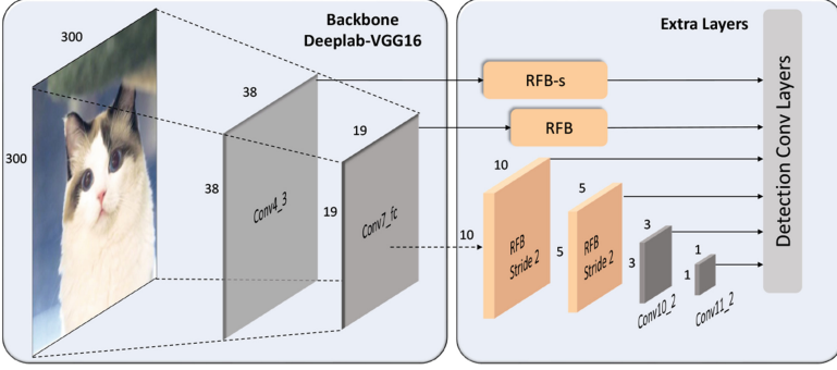
Fig. 5. The pipeline of RFB-Net300. The conv4.3 feature map is tailed by RFB-s which has smaller RFBs and an RFB module with stride 2 is produced by operating 2-stride multi-kernel conv-layers in the original RFB.
