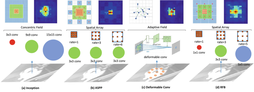
Fig. 3. Four typical structures of Spatial RFs. (a) shows the kernels of multiple sizes in Inception. (b) demonstrates the daisy-like pooling configuration in ASPP. (c) adopts deformable conv to produce an adaptive RF according to object characteristics. (d) illustrates the mechanism of RFB. The color map of each structure is the effective RF derived from one correspondent layer in the trained model, depicted by the same gradient back-propagation method in [23]. In (a) and (b), we adjust the RF sizes in original Inception and ASPP for fair comparison.
