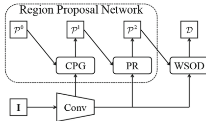
Fig. 1. The overall network architecture. “ I ”: input image; “ \mathcal{P}^0 ”: the initial proposals by sliding window, “ \mathcal{P}^1 ”: the proposals from the first stage of the network, “ \mathcal{P}^2 ”: the proposals from the second stage of the network, “ D ”: the detection results, “ Conv ”: convolutional layers, “ CPG ”: coarse proposal generation, “ PR ”: proposal refinement, “ WSOD ”: weakly supervised object detection
