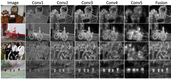
Fig. 2. The responses of different convolutional layers from the VGG16 [36] network trained on the ImageNet [32] dataset using only image-level annotations. Results from left to right are original images, response from the first to the fifth layers, and the fusion of responses from the second layer to the fourth layer
