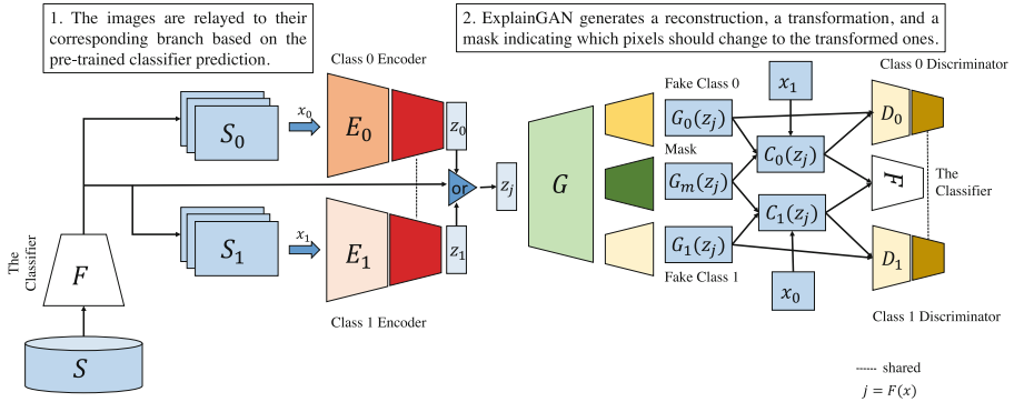
Fig. 1. Model architecture of ExplainGAN. Inference (in blue frame) consists of passing an image x of class j into the appropriate encoder E_j to produce a hidden vector z_j . The hidden vector is decoded to simultaneously create its reconstruction G_j(z_j) , a transformed image of the opposite class G_{1-j}(z_j) and a mask showing where the changes were made G_m(z_j) . Composite images C_0 and C_1 merge the reconstruction and transformation with the original image x . (Color figure online)
