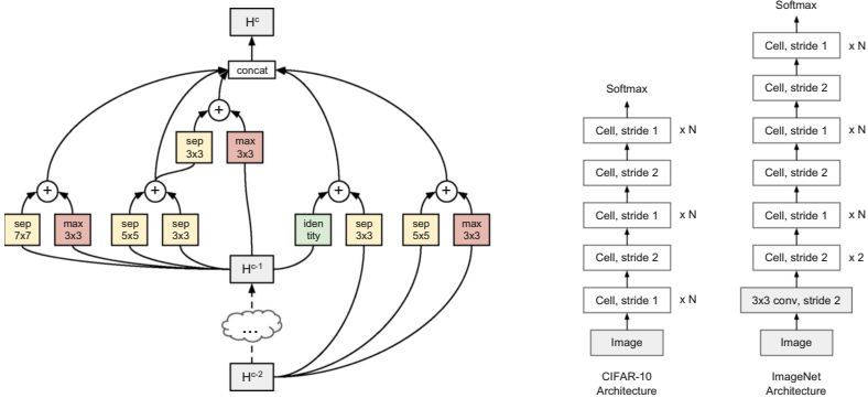
Fig. 1. Left: The best cell structure found by our Progressive Neural Architecture Search, consisting of 5 blocks. Right: We employ a similar strategy as [41] when constructing CNNs from cells on CIFAR-10 and ImageNet. Note that we learn a single cell type instead of distinguishing between Normal and Reduction cell.
