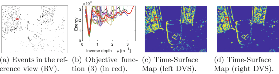
Fig. 3. Proposed objective function. (a) A randomly selected event, at pixel \mathbf{x} , is marked by a red circle in the reference view. The energy C(\mathbf{x}, \rho) in (3) is visualized in (b) as a function of \rho , with the thick red curve obtained by averaging the costs C(\mathbf{x}_i, \rho) of neighboring pixels \mathbf{x}_i in a patch centered at \mathbf{x} (indicated by curves with random colors). The vertical dashed line (black) indicates the ground truth inverse depth. The time-surface maps of the left and the right event cameras at one of the observation times are shown in (c) and (d), respectively, where the patches for measuring the temporal residual are indicated in red. (Color figure online)
