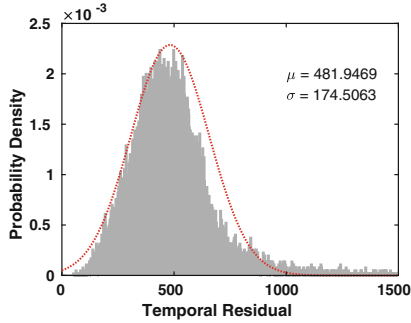
Fig. 4. Probability distribution (PDF) of the temporal residuals \{r_i\} : empirical (gray) and Gaussian fit \mathcal{N}(\mu, \sigma^2) (red line). (Color figure online)
