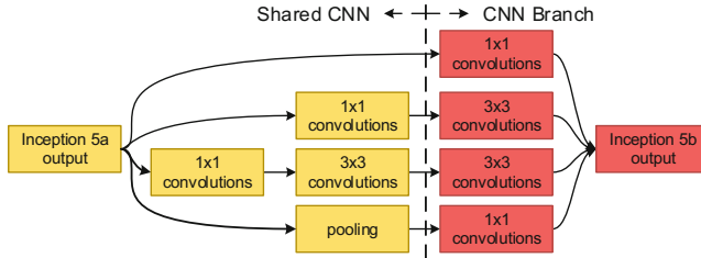
Fig. 4. The layers used in the shared CNN and CNN branches in the inception_5b block. The layers in yellow color are included in the shared CNN, while the layers in red color are duplicated for different branches. The layers after inception_5b are also duplicated. The ReLU and BatchNormalization layers after each convolutional layer are treated similarly as the corresponding convolutional layers. (Color figure online)
