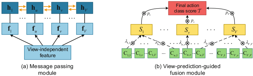
Fig. 3. The details for (a) inter-view message passing module discussed in Sect. 3.3, and (b) view-prediction-guided fusion module described in Sect. 3.4. Please see the corresponding sections for the detailed definitions and descriptions.
