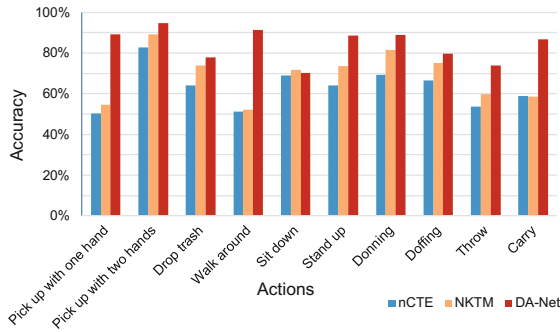
Fig. 5. Average recognition accuracy in each class on the NUMA dataset under the cross-view setting. All the three methods do not utilize the features from the unseen view during the training process.
