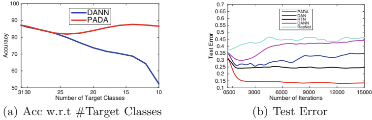
Fig. 5. Analysis: (a) Accuracy by varying #target domain classes; (b) Target test error.
