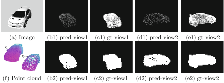
Fig. 3. (a) is the original image. (b1) & (d1) show the high resolution 2D projection of predicted point cloud in two different views. (c1) & (e1) show the high resolution 2D projection of the ground-truth point cloud. (b2)–(e2) show the corresponding low resolution results. (f) shows the ground-truth and predicted point cloud.
