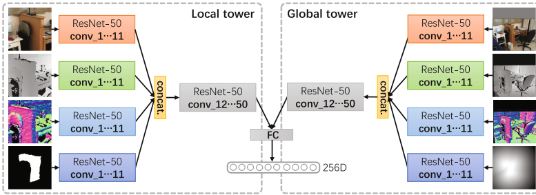
Fig. 3. Network architecture of the local and global towers. Layers shaded in the same color share weights. (Color figure online)
