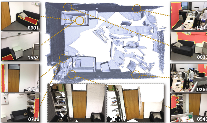
Fig. 1. Scene reconstruction based on coplanarity matching of patches across different views (numbers indicate frame ID) for both overlapping (left two pairs) and non-overlapping (right two pairs) patch pairs. The two pairs to the right are long-range, without overlapping. The bottom shows a zoomed-in comparison between our method (left) and key-point matching based method [2] (right).
