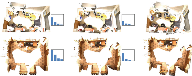
Fig. 9. Reconstruction results with 100% (left column), 50% (middle) and 0% (right) of long-range coplanar pairs detected, respectively. The histograms of long-range coplanar patch pairs (count over patch distance (1–5 m)) are given.
