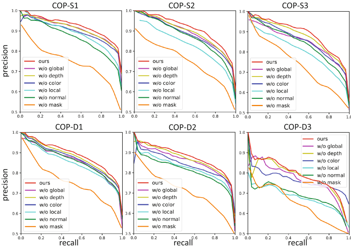
Fig. 7. Ablation studies of our coplanarity network.
