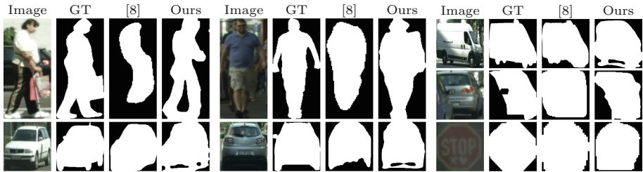
Fig. 5. Cityscapes mask comparison. From left to right: the original image, the ground truth mask (GT), the mask predicted by Simple Does It [8], and our mask.
