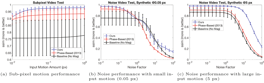
Fig. 8. Quantitative analysis. (a) Subpixel test, our network performs well down to 0.01 pixels, and is consistently better than the phase-based [24]. (b, c) Noise tests at different levels of input motion. Our network’s performance stays high and is consistently better than the phase-based whose performance drops to the baseline level as the noise factor exceeds 1. Our performance in (b) is worse than (c) because the motion is smaller, which is expected because a smaller motion is harder to be distinguished from noise.
