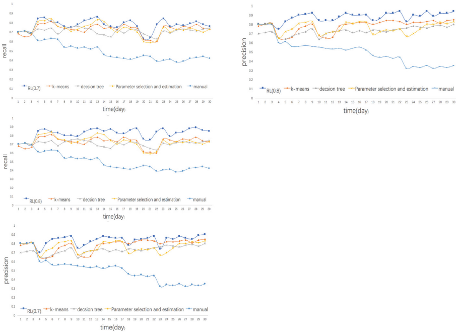
Fig. 6. Comparison of recall and precision
