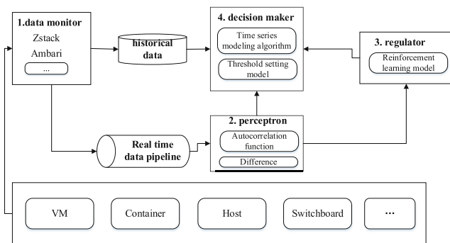
Fig. 1. Anomaly detection framework
