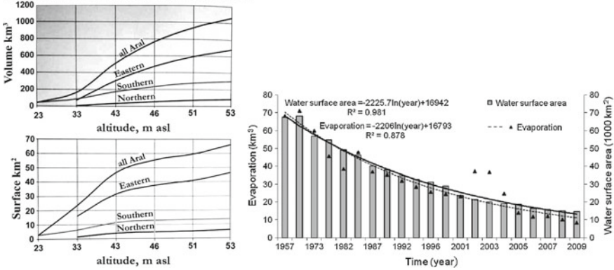
Fig. 5.2 Left: Aral Sea morphometry (source Nazionalnyi Atlas Respubliki KZ 2010). Right: evolution of water surface and evaporation volumes, 1957–2009 (source Gaybullayev and Chen 2012)
