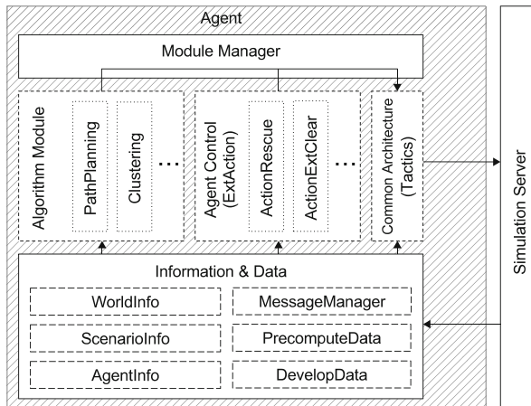
Fig. 4. Structure of framework
