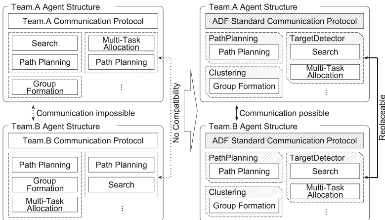
Fig. 2. Before and after introducing common architecture
