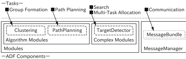
Fig. 3. Relationship between RRS tasks and ADF components
