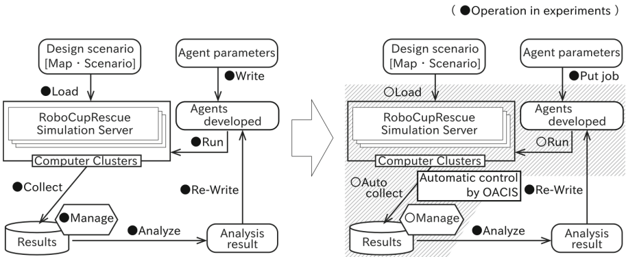
Fig. 5. Before and after introducing experimental management by OACIS
