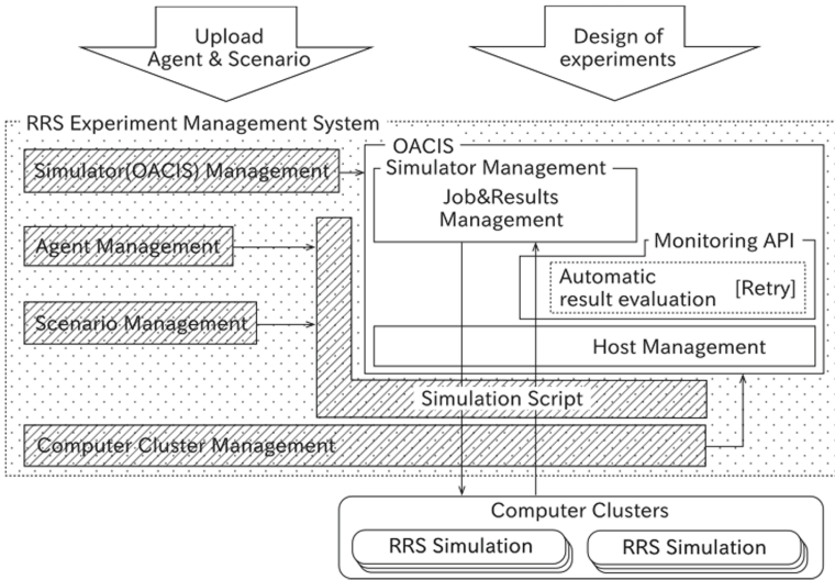
Fig. 6. Extensions of OACIS for RRS
