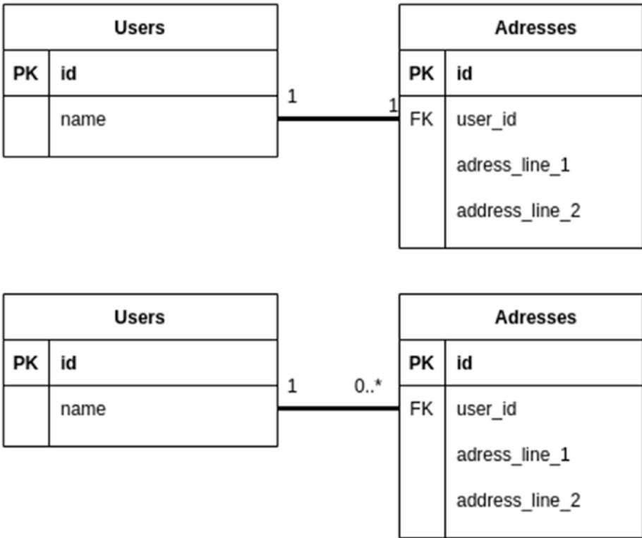
Figure 9-7. ERD
