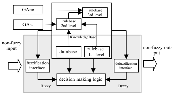
Fig. 1. GF-Miner architecture
