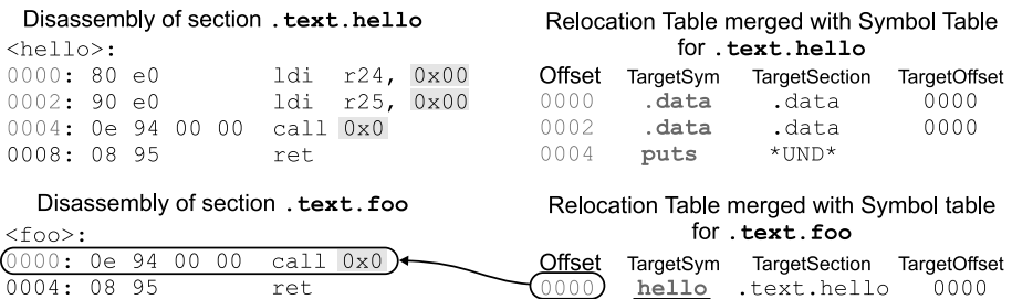
Figure 4. The relocation information shows that foo needs hello. If we update hello and thereby move it to a new position we need to modify foo as well.
