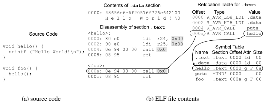
Figure 3. Example of the contents in an ELF file and its relationship
