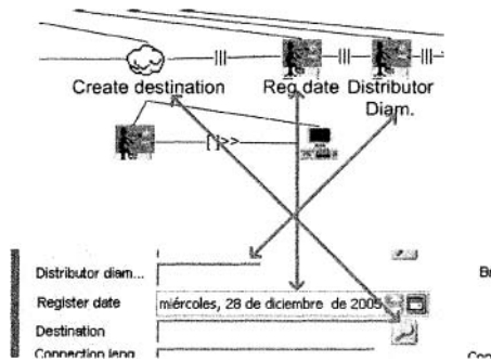
Fig. 7. Correspondences between CTT and the final widgets
