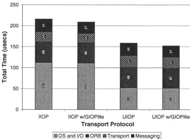
Figure 6 Comparison of ORB and Transport/OS Overhead Using Timeprobes
