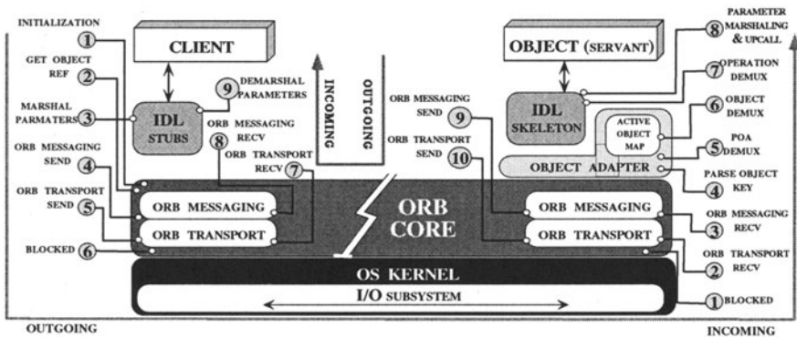
Figure 5 Timeprobe Locations for Whitebox Experiment
