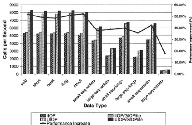
Figure 4 TAO's Pluggable Protocols Framework Performance Over Local IPC and TCP/IP
