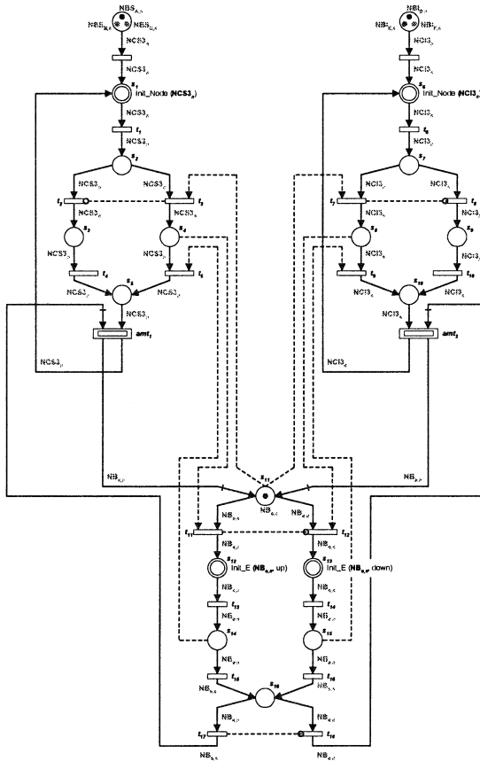
Figure 6: A shobi-PN v2.0 specification net.
