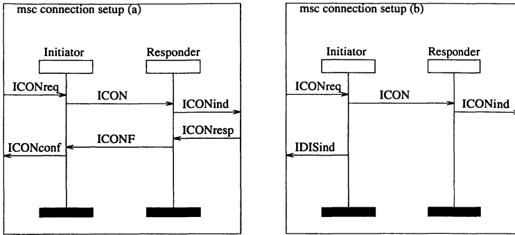
Figure 1. Two Message Sequence Charts
