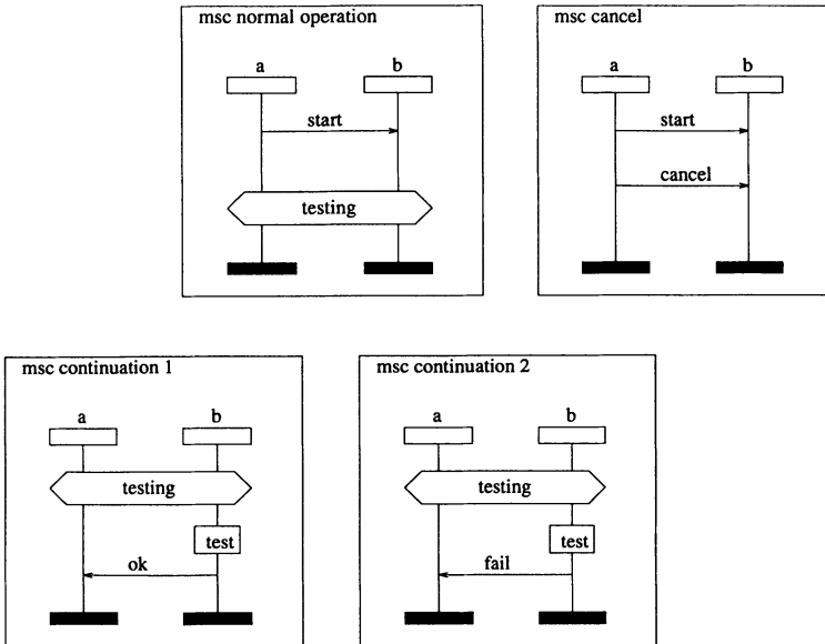
Figure 3. Example Message Sequence Charts
