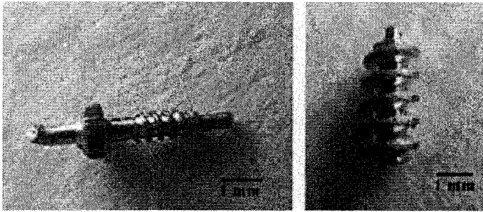
Fig. 3. Examples of micro work pieces manufactured with the first micromachine tool prototype
