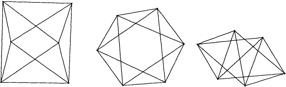
Fig. 16. Three different layouts of an octahedron ( |V| = 6 , |E| = 12 ) after \leq 200 iterations
