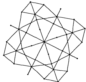
Fig. 19. GEM drawing of the graph in [3, fig. 12]; this drawing is similar to [6, fig. 26]
