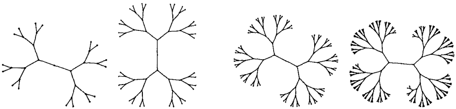
Fig. 10. Binary trees of size |V| = 31, 63, 127, 255 after 1178, 3276, 9906, 34935 iterations
