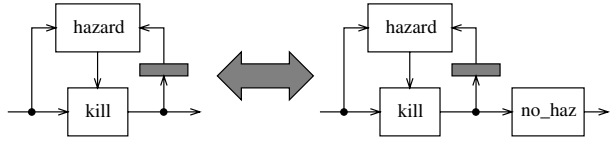
Fig. 9. Hazard-squashing logic guarantees no hazards
