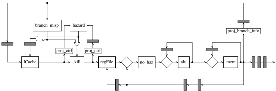
Fig. 11. Microarchitecture after the “propagate hazard information” step
