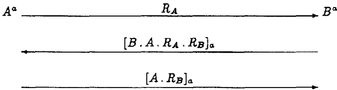
Fig. 1. Protocol MAP1: a mutual authentication of any two principals, A and B , among a set of principals I who share a key a .
