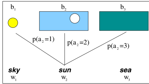
Fig. 2. Notation
