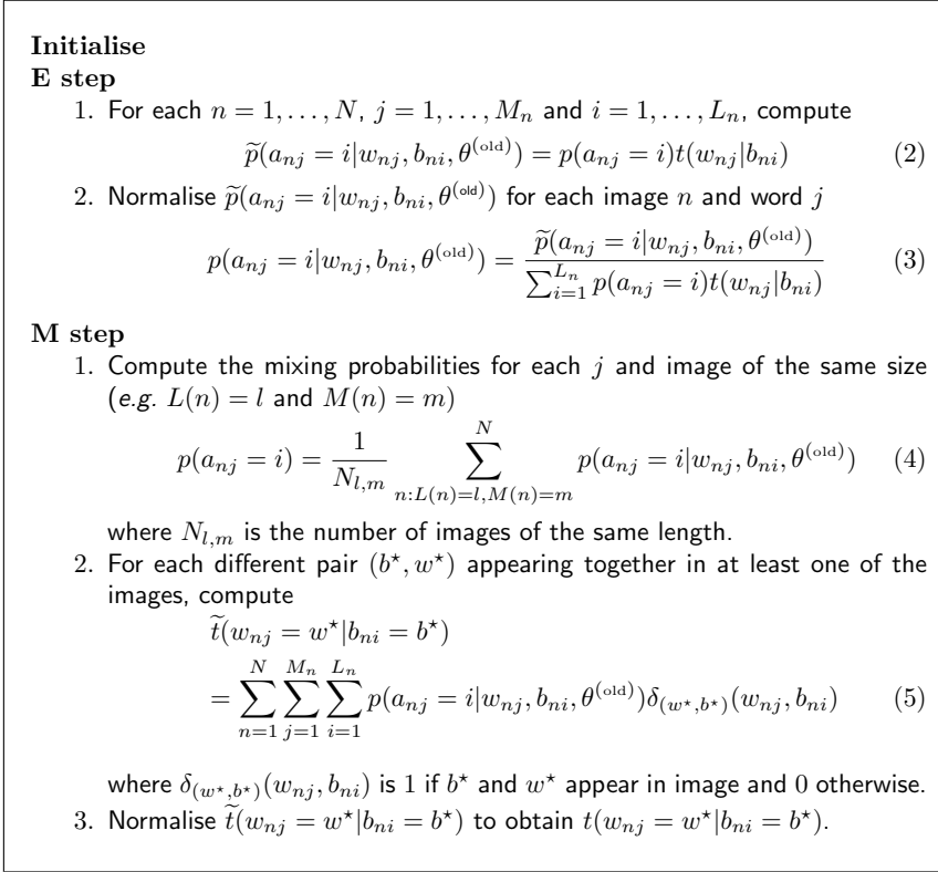
Fig. 4. EM (Expectation Maximization) algorithm
