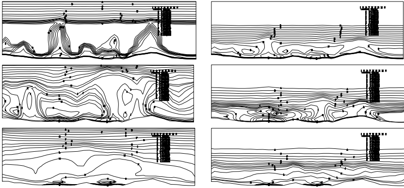
Fig. 4. Potential temperature distributions at characteristic location where both residential and industrial zone are present, for different time instants, \tau=1 p.m., 6 p.m. (day I), 10 a.m. (day II): left- weak stratification, right- strong stratification.
