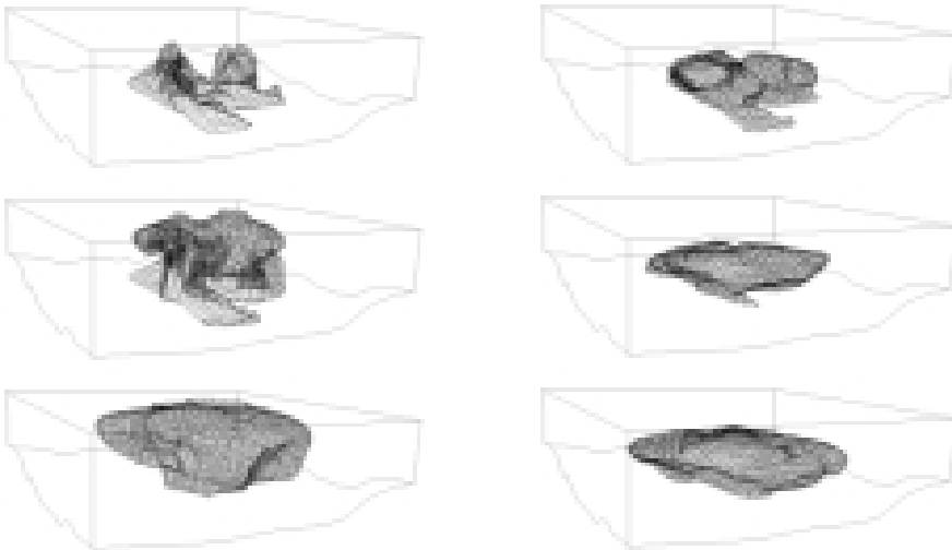
Fig. 8. Time evolution of concentration ( \langle C \rangle = 0.01 ), \tau = 1 p.m., 6 p.m., day (I), 10 p.m., day (II) respectively; left- weak stratification, right- strong stratification.
