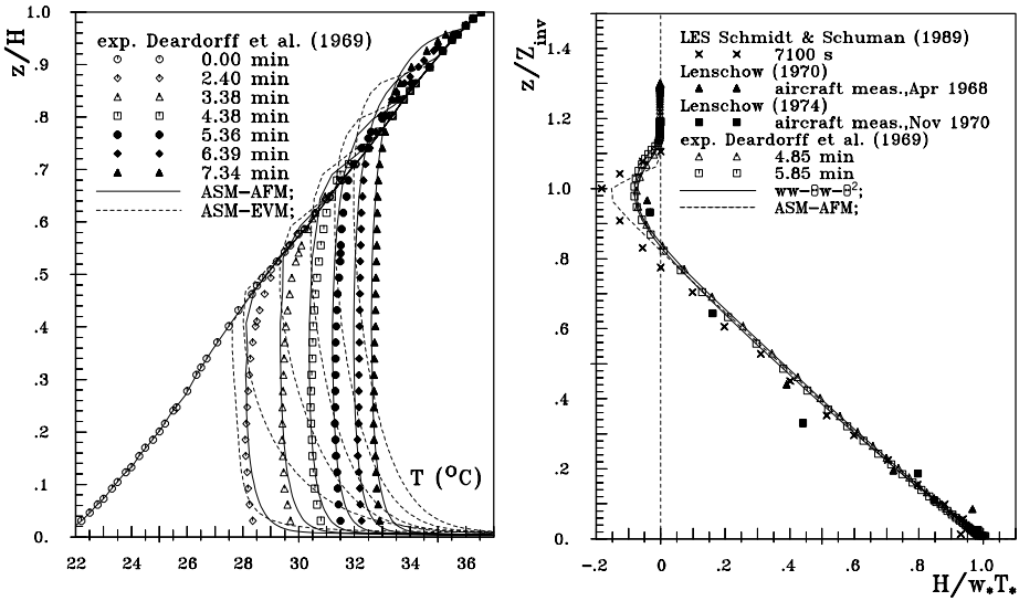
Fig. 1. Time evolution of vertical temperature profiles in a mixed layer heated from below -left, Normalised vertical heat flux in a mixed layer heated from below- right: comparison between experiments and simulations.
