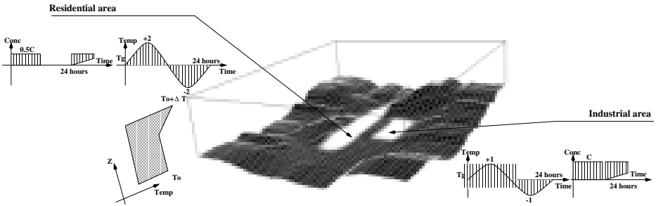
Fig. 3. Specification of imposed boundary and initial conditions for a middle-size town located in a mountain area; Two distinct areas (industrial and residential) are represented by different pollution emission ( C = 100 and 50\% respectively) and different heat source intensities ( T_g = \pm 1 and \pm 2 respectively); Initial thermal stratification is also presented.
