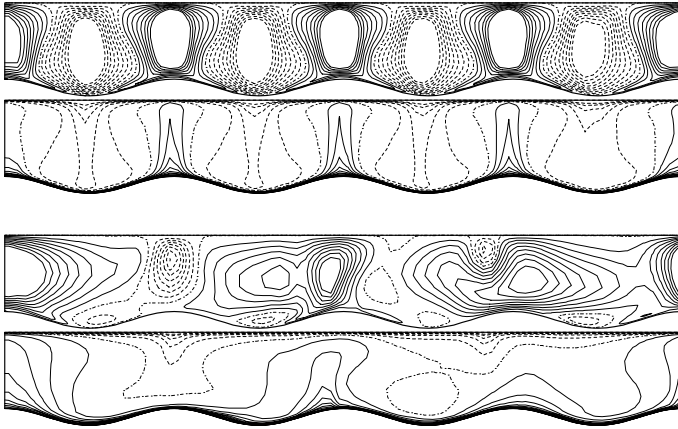
Fig. 2. Vertical velocity \langle W \rangle and temperature \langle T \rangle distributions in turbulent thermal convection over a terrain with 3D regular waviness, S_B(x, y) = 0.1 \cos(x\pi) \cos(y\pi) , Ra=10^7 , Pr=0.71 ; above- \tau^*=50 , below- \tau^*=200 .
