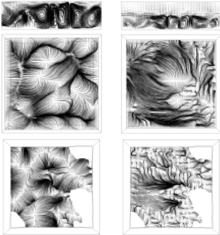
Fig. 6. Instantaneous trajectories in characteristic vertical plane (over residential and industrial zones) and two horizontal planes: first- at the base of inversion layer, second- 50m from ground; \tau=6 p.m., day II, case with weak stratification: left- weak stratification, right- strong stratification.
