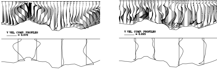
Fig. 7. Velocity vectors and horizontal velocity component profiles indicating an inertial motion, 2hrs after onset of heating/cooling, day (II), case with weak stratification: left- up-slope motion, right- down-slope motion.
