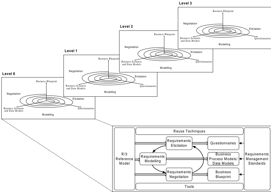
Fig.2. The SAP requirements engineering process
