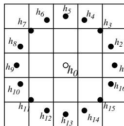
Fig. 3. The circularly symmetric neighbor set of 16 pixels in a 5x5 neighborhood.
