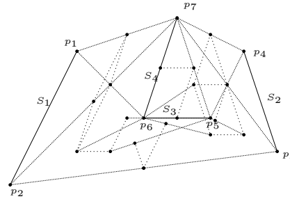
Fig. 9. A reflection-visibility partition
