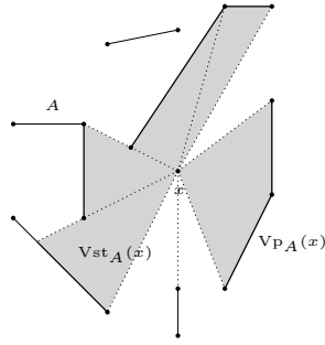
Fig. 4. A visibility star
