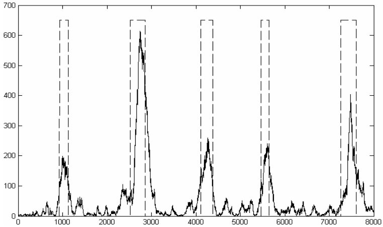
Fig. 1. Plot of laA + tT + cC + gG^2 for the 8000 bp stretch starting at position 7020 inside Chromosome III of C. elegans , using a sliding window of length 351. Noticeable peaks correspond to coding regions, which are represented using dashed lines.
