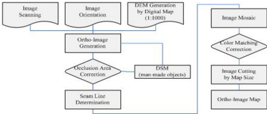
Fig. 1. The proposed scheme for true ortho-image production
