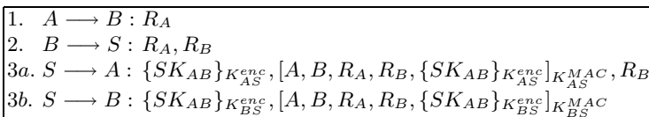
Fig. 5. Choo, Boyd, Hitchcock, & Maitland provably secure 3PKD protocol
