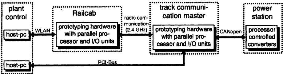
Figure 2: The Railcab system test track
