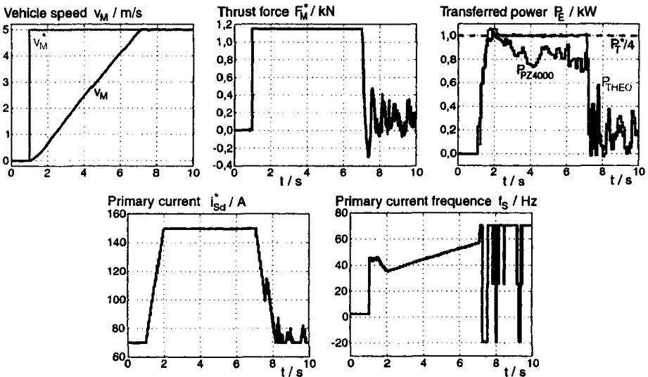
Figure 5: Step response of speed control with control of energy transfer
