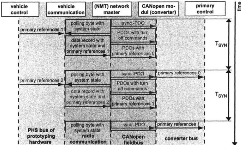
Figure 3: Diagram of communication sequences
