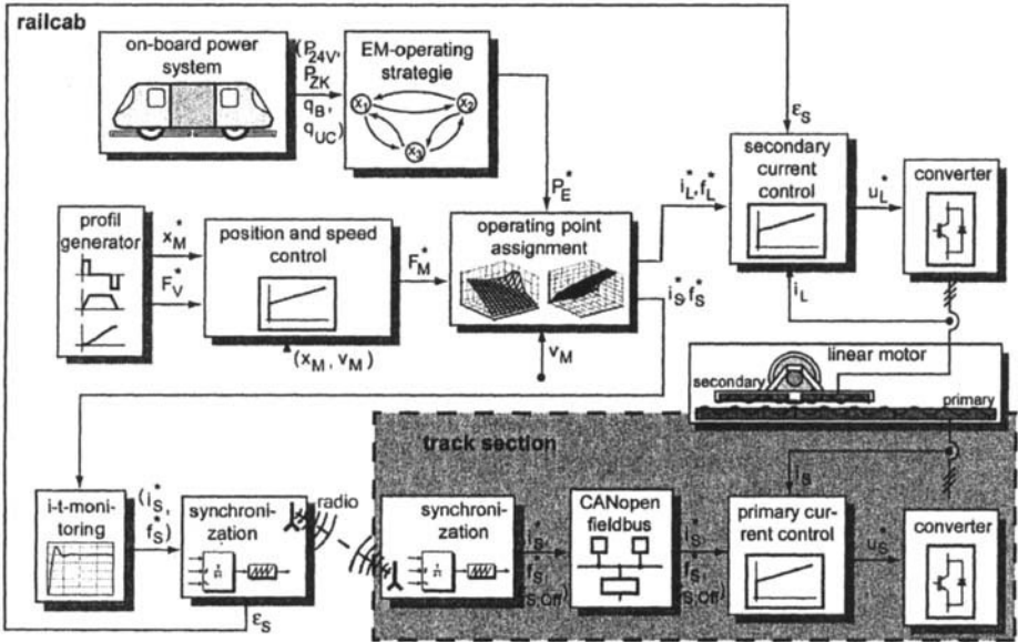
Figure 4: Linear drive control structure
