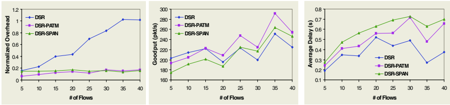
Fig. 9. Performance Comparison between PATM and SPAN
