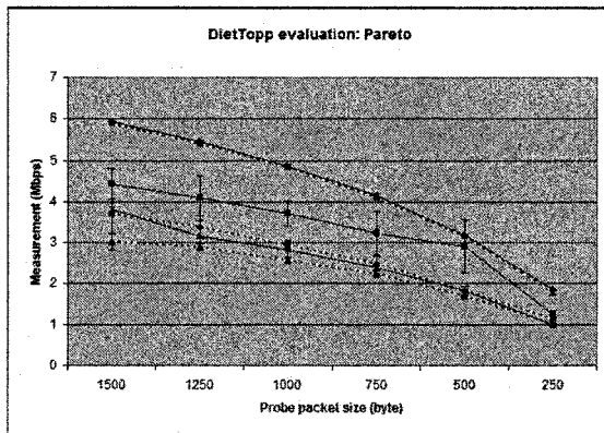
Figure 6. Available bandwidth (dashed lines) and measured link capacity (solid lines) measured under 0, 250 Kbps and 500 Kbps pareto distributed cross-traffic.
