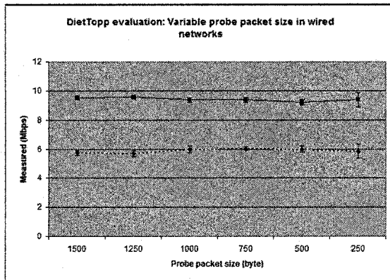
Figure 4. Available bandwidth (dashed line) and link capacity (solid line) measured by DietTopp in a wired network using different probe packet sizes. The cross traffic is a 3.26 Mbps pareto distributed stream on a 10 Mbps link.
