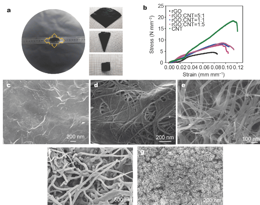
Figure 1 (a) Photographs, (b) tensile strain-stress curves and (c–e) SEM images of large-scale robust nanocarbon films, (f) SEM image, (g) high-magnification SEM image of rGO/CNT/MnO x film.
